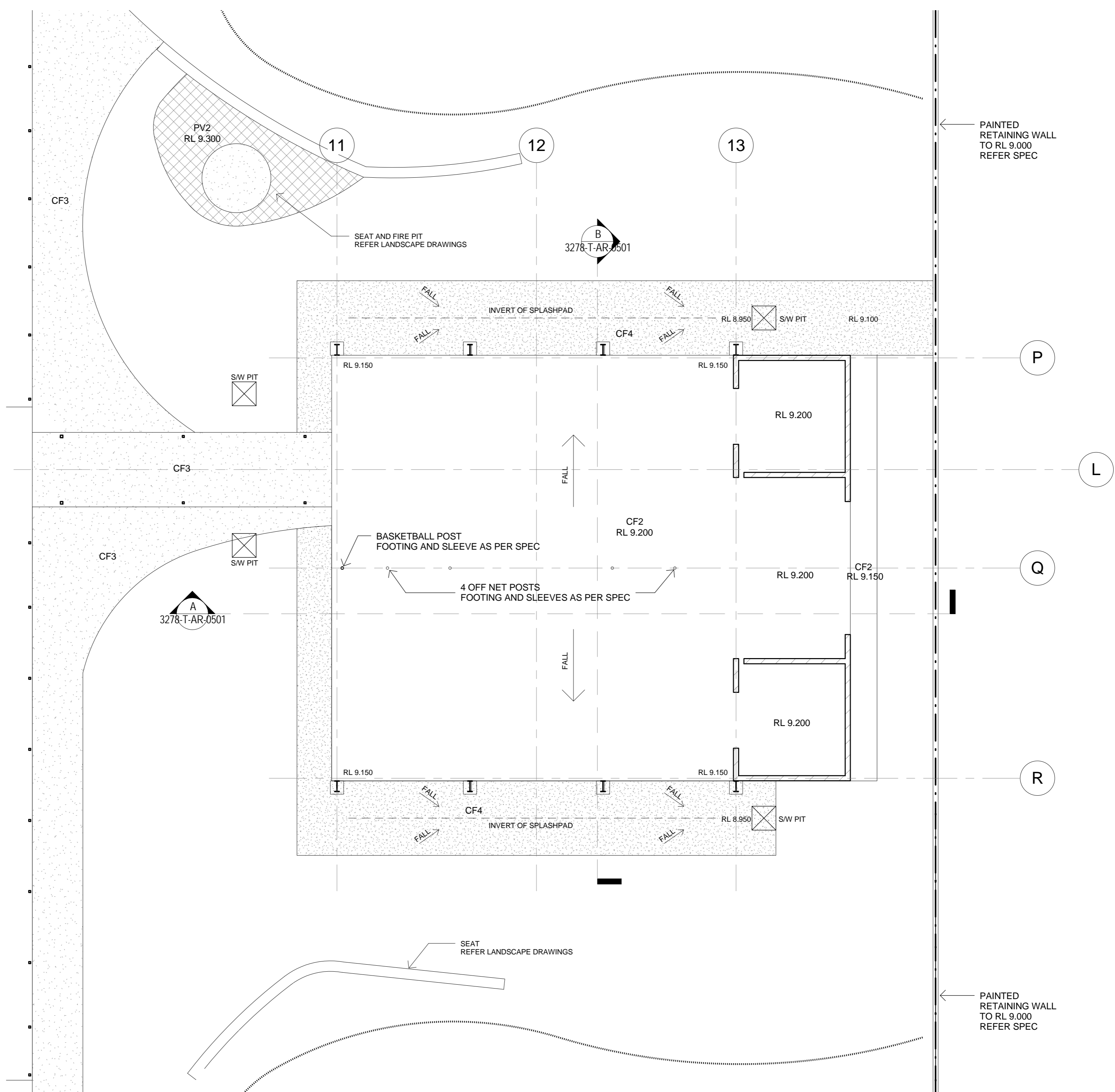
COVERED AREA - GROUND FLOOR STRUCTURAL SETOUT
