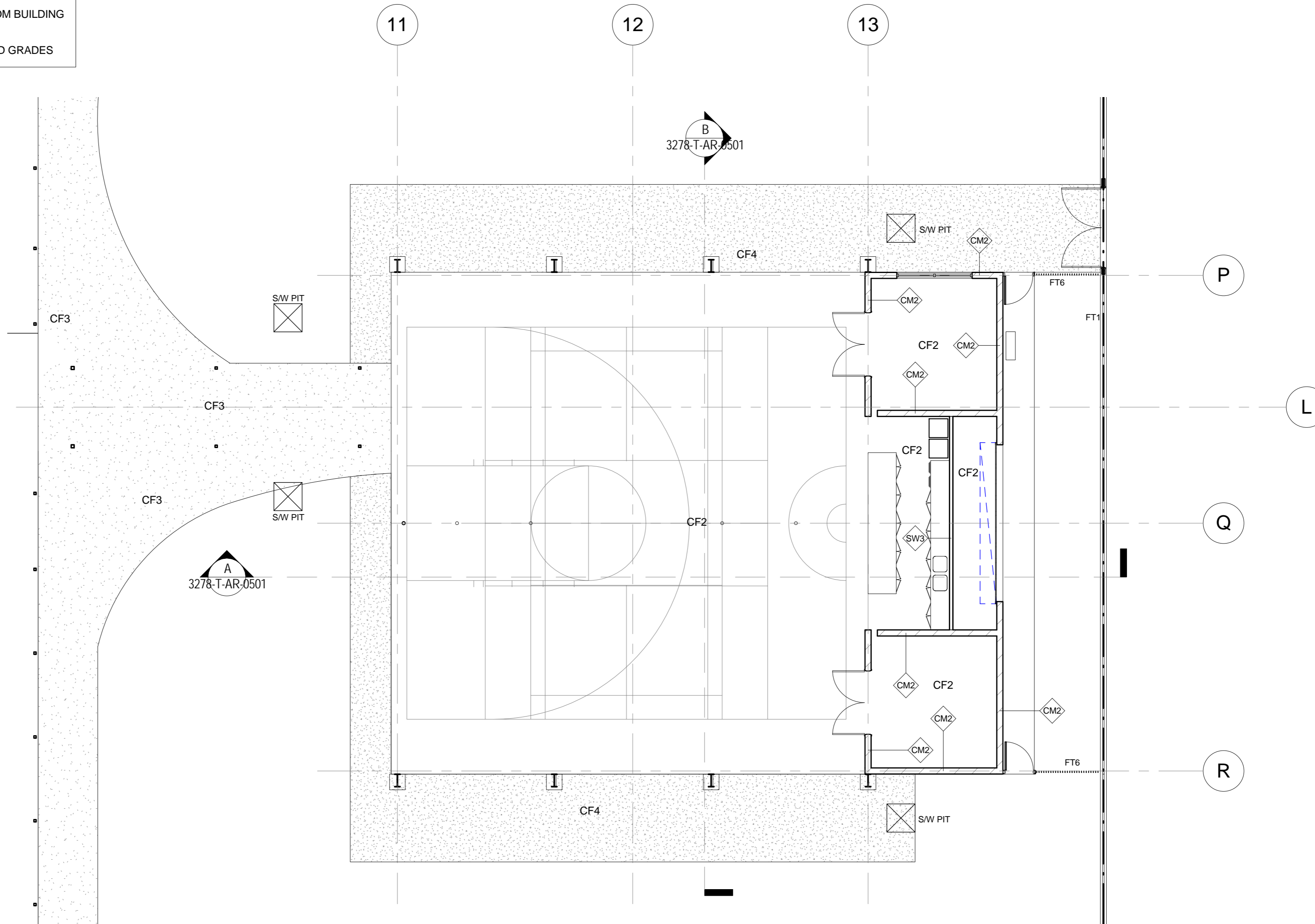
COVERED AREA - GROUND FLOOR FINISHES
